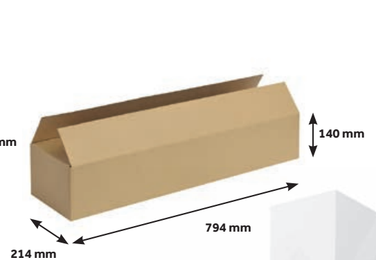
WPS794X214X140HHB
